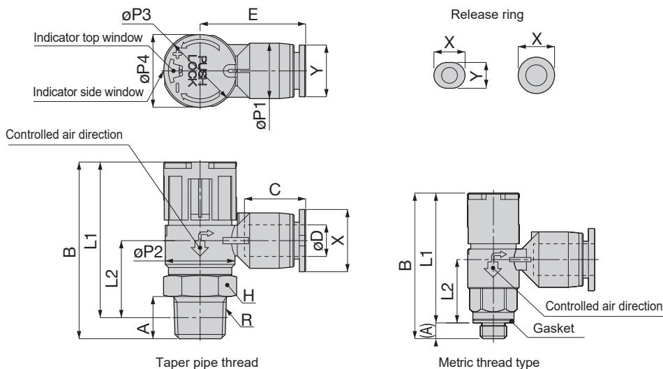
Meter-out control (Air supply control)
