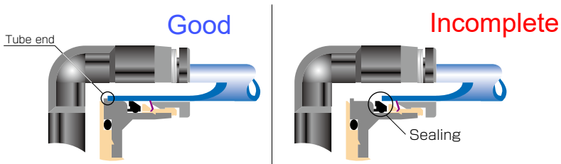
Tube is not fully inserted up to tube end.
